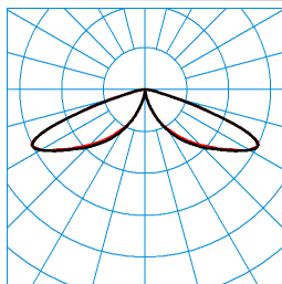
LTX PT-RB6L-LRA/15/18/26-730 4G1 (1500 lm) TX084170 ■ C0 - C180 ■ C90 - C270 DIN 5040: A20 UTE: 1,00 J CEN Flux Code: 15 51 95 100 100 0 0 0 0
