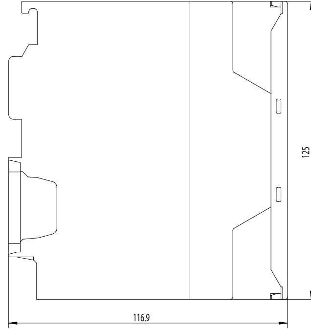
Links / Left
