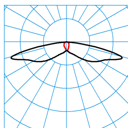
Jovie 50-SB3L-LRA/1350-740 2G1 ET (CLO initial value) TX301406 ■ C0 - C180 ■ C90 - C270 DIN 5040: A20 UTE: 1,00 l CEN Flux Code: 29 61 91 100 100
