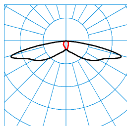
Jovie 50-SB3L-LRA/1350-740 2G1 ET (CLO end value) TX300377 ■ C0 - C180 ■ C90 - C270 DIN 5040: A20 UTE: 1,00 l CEN Flux Code: 29 61 91 100 100
