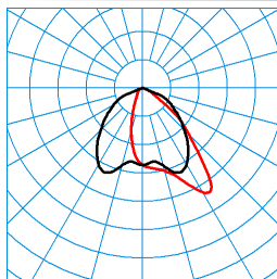
Jovie 70I-AM3L-SLR2/24000-730 24G1 ET TX195575 ■ C0 - C180 ■ C90 - C270 DIN 5040: A50 UTE: 1,00 D CEN Flux Code: 59 89 100 100 100
