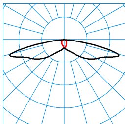
Jovie 50-SB3L-LR/1350-730 2G1 ET (CLO initial value) TX301076 ■ C0 - C180 ■ C90 - C270 DIN 5040: A20 UTE: 1,00 l CEN Flux Code: 29 61 91 100 100
