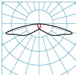
Jovie 50-SB3L-LR/1350-730 2G1 ET (CLO end value) TX301455 ■ C0 - C180 ■ C90 - C270 DIN 5040: A20 UTE: 1,00 l CEN Flux Code: 29 61 91 100 100
