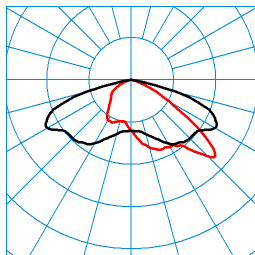
LnPlus 40-AB7L/13500-730 12G1 ETDD (CLO initial value) TX377760 ■ C0 - C180 ■ C90 - C270 DIN 5040: A30 UTE: 1,00 G CEN Flux Code: 35 73 98 100 100
