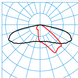
LIQ 50N-AB2L-SLR1/4200-740 4G1 ET (CLO end value) TX278030 ■ C0 - C180 ■ C90 - C270 DIN 5040: A30 UTE: 1,00 G CEN Flux Code: 34 71 96 100 100 0 0 0 0
