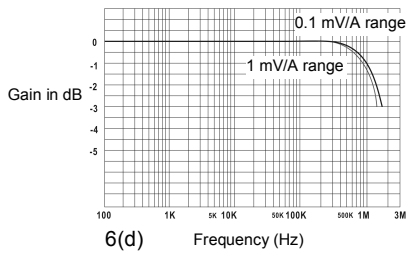
Figure 6(a – d): Gain versus Frequency @ 1 A peak, typical
