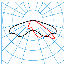
LIQ 90-AB7L-SLR1/29000-740 24G1S TX122194 ■ C0 - C180 ■ C90 - C270 DIN 5040: A30 UTE: 1,00 l CEN Flux Code: 33 72 98 100 100
