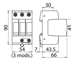
Dimensions DG M WE 600
