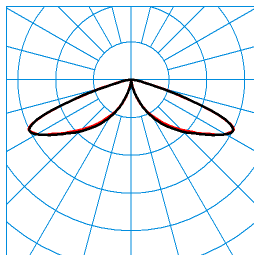
LTX ZT-RB6L-LRA/15/18/26-730 4G1 (1800 lm) TX084224 ■ C0 - C180 ■ C90 - C270 DIN 5040: A20 UTE: 1,00 J CEN Flux Code: 15 51 96 100 100 0 0 0 0
