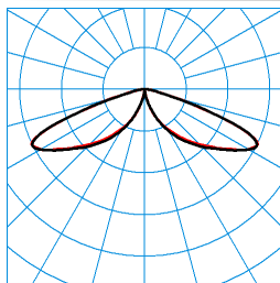
LTX ZT-RB6L-LRA/15/18/26-730 4G1 (1500 lm) TX084223 ■ C0 - C180 ■ C90 - C270 DIN 5040: A20 UTE: 1,00 J CEN Flux Code: 15 51 95 100 100 0 0 0 0
