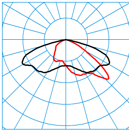
LnPlus 40-AB7L/6200-740 12G1 ETDD (CLO initial value) TX376865 ■ C0 - C180 ■ C90 - C270 DIN 5040: A30 UTE: 1,00 G CEN Flux Code: 35 73 98 100 100
