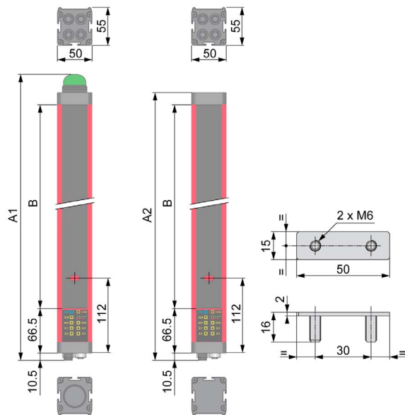
Safety light curtain dimensions and weights for XUSL4M with 2/3/4 beams:
