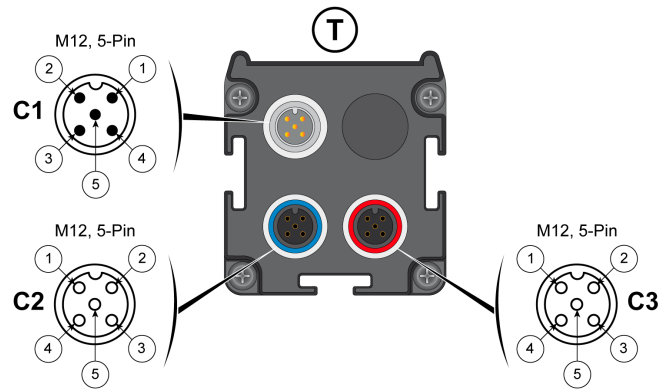
C1 - GRAY CONNECTOR - Range/Test selection male connector (M12, 5-Pin):
