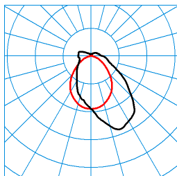
TugraHE 9 PAW 18-56/16ML-840 ET PC 23 (STAG13) TX425172 C0 - C180 C90 - C270 DIN 5040: B40 UTE: 0,86 E + 0,14 T CEN Flux Code: 48 77 92 86 100 13 32 64 14
