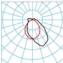
TugraHE 9 PAW 18-56/16ML-840 ET PC 23 (STAG10) TX425147 C0 - C180 C90 - C270 DIN 5040: B40 UTE: 0,86 E + 0,14 T CEN Flux Code: 48 77 92 86 100 13 32 64 14
