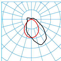
TugraHE 9 PAW 18-56/16ML-840 ET PC 23 (STAG12) TX425219 C0 - C180 C90 - C270 DIN 5040: B40 UTE: 0,86 E + 0,14 T CEN Flux Code: 48 77 92 86 100 13 32 64 14
