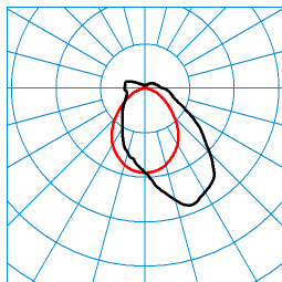
TugraHE 9 PAW 18-56/16ML-840 ET PC 23 (STAG11) TX425052 C0 - C180 C90 - C270 DIN 5040: B40 UTE: 0,86 E + 0,14 T CEN Flux Code: 48 77 92 86 100 13 32 64 14
