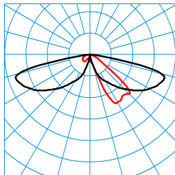
LTX P-AB2L-LRA/15/18/26-740 4G1 (1500 lm) TX059699 ■ C0 - C180 ■ C90 - C270 DIN 5040: A20 UTE: 1,00 l CEN Flux Code: 24 61 92 100 100 0 0 0 0
