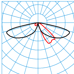
LTX P-AB2L-LRA/15/18/26-740 4G1 (2600 lm) TX062702 ■ C0 - C180 ■ C90 - C270 DIN 5040: A20 UTE: 1,00 l CEN Flux Code: 24 61 92 100 100 0 0 0 0
