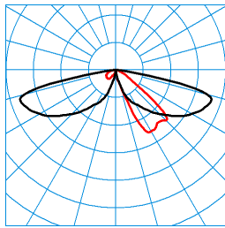
LTX P-AB2L-LRA/15/18/26-740 4G1 (1800 lm) TX062701 ■ C0 - C180 ■ C90 - C270 DIN 5040: A20 UTE: 1,00 l CEN Flux Code: 24 61 92 100 100 0 0 0 0
