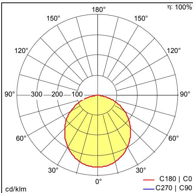
D36853AA_u_ONDA2_E_D590_LED5800-830.ltd
