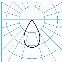
E-Line 7751 B.VEO RFS-VFL-c 05 20-M J05 ETDD L37 03 ■ C0 - C180 TX095142
