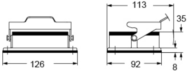
Catalogue drawings
