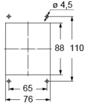
Catalogue drawings
