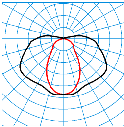
Acquex LED-M 1.5 60-840 ETDD PC TX375242
