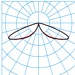
LTX KT-RB6L-LRA/15/18/26-730 4G1 (1800 lm) TX084065 ■ C0 - C180 ■ C90 - C270 DIN 5040: A20 UTE: 1,00 J CEN Flux Code: 15 51 96 100 100 0 0 0 0
