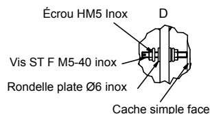
Fixation potence horizontale
