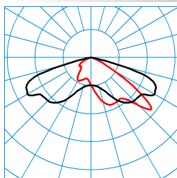
LIQ 90-AB7L-LR/20000-730 24G1S TX044831 ■ C0 - C180 ■ C90 - C270 DIN 5040: A30 UTE: 1,00 l CEN Flux Code: 33 72 98 100 100
