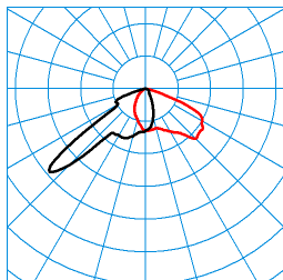
LIQ 70N-FL1L/9100-740 10G1 ET(CLO initial value) TX277814 ■ C0 - C180 ■ C90 - C270 DIN 5040: A40 UTE: 1,00 F CEN Flux Code: 43 84 100 100 100
