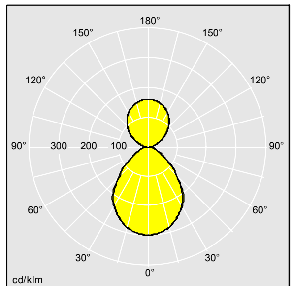
TL_PNC3_LRO_MSP_6600-940_L15_HF.ltd
