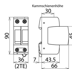
Dimensions DG M TN 275 NL
