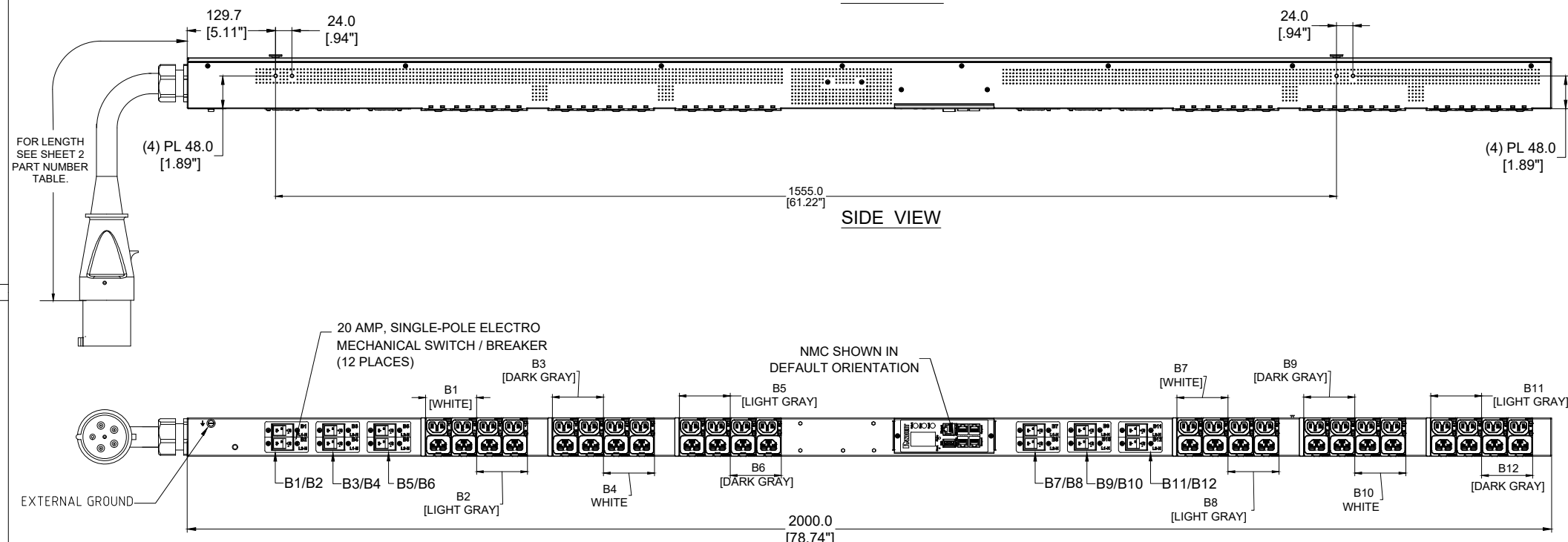
FRONT VIEW
