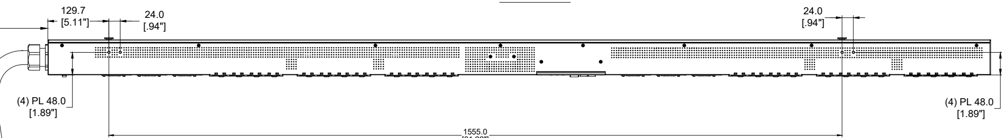
SIDE VIEW
