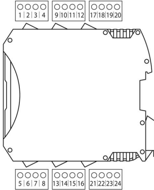
Module XPSMCMDO0016C1•
