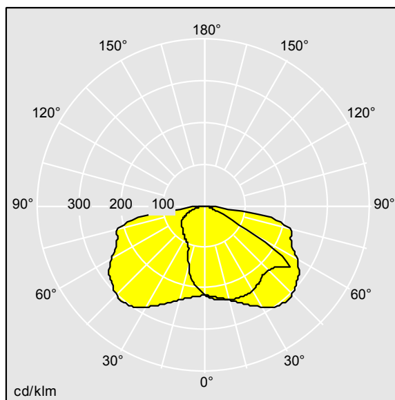
TL_CQL60L35EWS740.ltd
