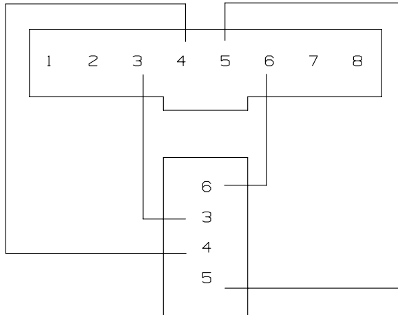
PORT WIRING SCHEME
