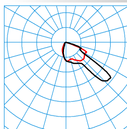
LIQ 50N-FR1L/5600-722 6G1 ET (CLO end value) TX281024 ■ C0 - C180 ■ C90 - C270 DIN 5040: A40 UTE: 1,00 F CEN Flux Code: 41 83 99 100 100
