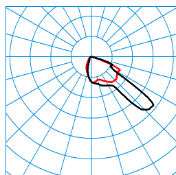
LIQ 50N-FR1L/5600-722 6G1 ET (CLO initial value) TX281096 ■ C0 - C180 ■ C90 - C270 DIN 5040: A40 UTE: 1,00 F CEN Flux Code: 41 83 99 100 100
