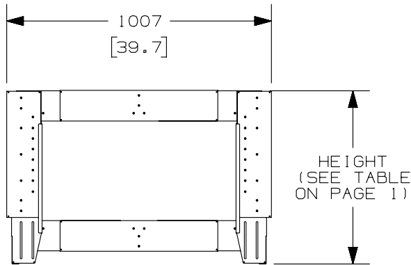
FRONT VIEW COLLAPSED
