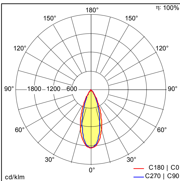
STx586.idt
