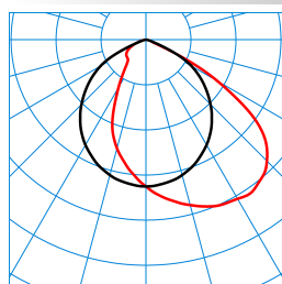
Combial 40 G2 AM9L/80-150/3/ML-MC G1 ET (stage 1) TX711706 ■ C0 - C180 ■ C90 - C270 DIN 5040: A50 UTE: 1,00 D DLOR: 100 % ULOR: 0 % CEN Flux Code: 54 88 99 100 100
