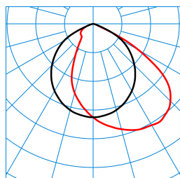
Combial 40 G2 AM9L/80-150/3/ML-MC G1 ET (stage 3) TX711710 ■ C0 - C180 ■ C90 - C270 DIN 5040: A50 UTE: 1,00 D DLOR: 100 % ULOR: 0 % CEN Flux Code: 54 88 99 100 100
