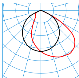
Combial 40 G2 AM9L/80-150/3/ML-MC G1 ET (stage 2) TX711694 ■ C0 - C180 ■ C90 - C270 DIN 5040: A50 UTE: 1,00 D DLOR: 100 % ULOR: 0 % CEN Flux Code: 54 88 99 100 100
