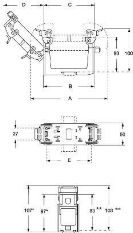
Catalogue drawings
