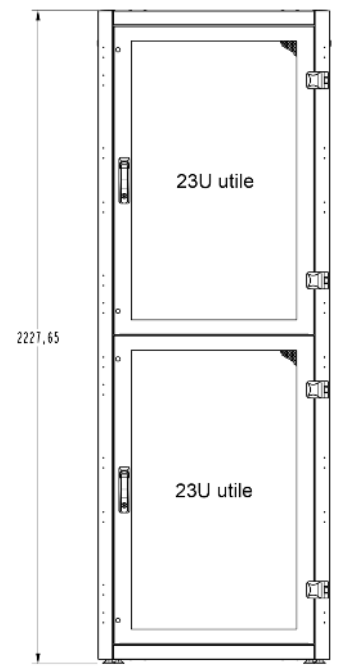
C2 - 47U - 2 compartiments
