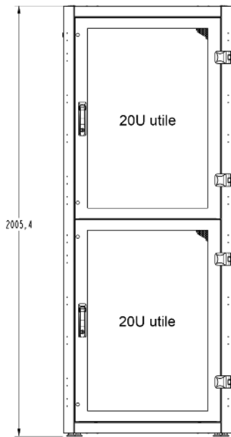
C2 - 42U - 2 compartiments
