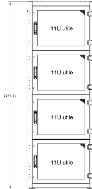
C2 - 47U - 4 compartiments
