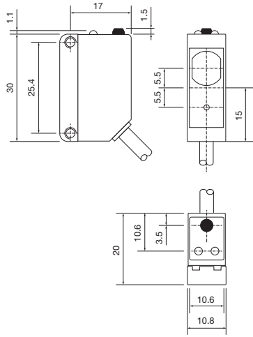
LD30EPBRxxBPA2IO
