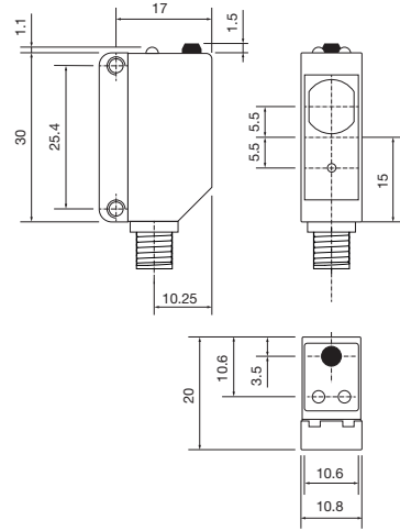
LD30EPBRxxBPM5IO
