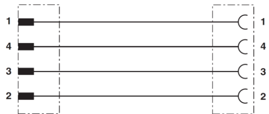
Wiring diagram
