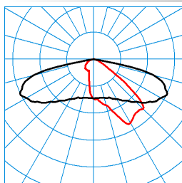
LIQ 50N-AB2L-LR/2200-740 4G1 ET (CLO end value) TX278207 ■ C0 - C180 ■ C90 - C270 DIN 5040: A30 UTE: 1,00 G CEN Flux Code: 34 71 96 100 100 0 0 0 0
