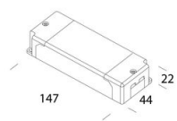
Driver 700mA
