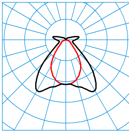
TugraHE Act 18 PW19 50 ETDD8 01 (ACTDCW) TX375149 ■ C0 - C180 ■ C90 - C270 DIN 5040: B41 UTE: 0,81 D + 0,19 T CEN Flux Code: 60 85 94 81 100 9 28 64 19
