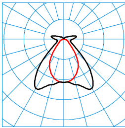
TugraHE Act 18 PW19 50 ETDD8 01 (ACTDWW) TX375151 ■ C0 - C180 ■ C90 - C270 DIN 5040: B41 UTE: 0,81 D + 0,19 T CEN Flux Code: 60 85 94 81 100 9 28 64 19
