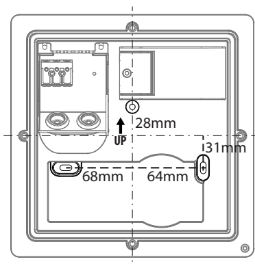
Frame Square/Wall
