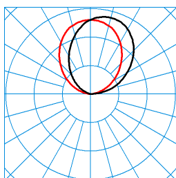
Sanesca W2 LED5000-830 01 (room light) TX055756 DIN 5040: E03 UTE: 0,00 J + 1,00 T CEN Flux Code: 0 0 0 0 100 50 81 96 100
