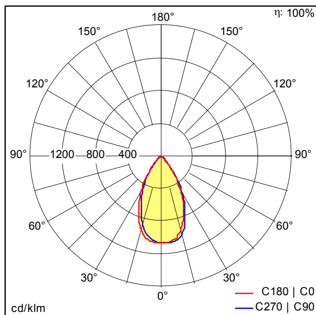
TE_LILY_LED_SPOT_IP44_60_68_600_930.ltd
