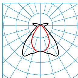
TugraHE Act 15 PW19 50 ETDD8 01 (ACTDSU) TX303455 ■ C0 - C180 ■ C90 - C270 DIN 5040: B41 UTE: 0,81 D + 0,19 T CEN Flux Code: 60 85 94 81 100 9 28 64 19
