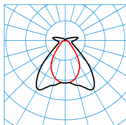
TugraHE Act 15 PW19 50 ETDD8 01 (ACTDCW) TX302672 ■ C0 - C180 ■ C90 - C270 DIN 5040: B41 UTE: 0,81 D + 0,19 T CEN Flux Code: 60 85 94 81 100 9 28 64 19
