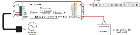
3. Connect with single color LED lighting
