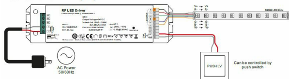
1. Connect with RGBW LED lighting
