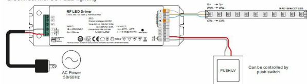
2. Connect with CCT LED lighting
