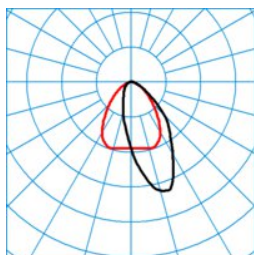
ELINE HE LAN40-120 ML 840 L150 2 20 ■ C0 - C180
