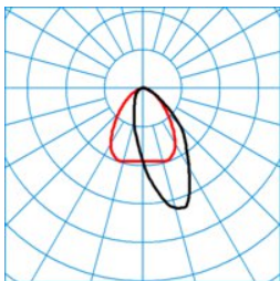
ELINE LAN40-110 ML 840 L150 4 20 ■ C0 - C180 DIN 5040 3 = A50 UTE 3 = 0.98 C + 0.02 T CEN flux code = 63 89 98 98 100 0 6 44 2
