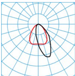
ELINE LAN40-110 ML 840 L150 0 20 ■ C0 - C180 DIN 5040 = A50 UTE 3 = 0.98 C + 0.02 T CEN flux code = 63 89 98 98 100 0 6 44 2
