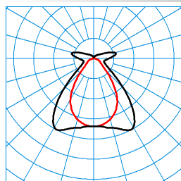
TugraHE Act 9 PW19 30 ETDD8 01 (ACTDWW) TX302552 ■ C0 - C180 ■ C90 - C270 DIN 5040: B41 UTE: 0,81 D + 0,19 T CEN Flux Code: 60 85 94 81 100 9 28 64 19
