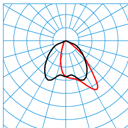
Jovie 70I-AM3L-SLR3/18000-740 18G1 ET (CLO initial value) TX300672 ■ C0 - C180 ■ C90 - C270 DIN 5040: A50 UTE: 1,00 D CEN Flux Code: 59 89 100 100 100
