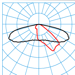
LIQ 50N-AB2L-SLR1/2200-730 2G1 ET (CLO end value) TX278336 DIN 5040: A30 UTE: 1,00 G CEN Flux Code: 34 71 96 100 100 0 0 0 0 ■ C0 - C180 ■ C90 - C270
