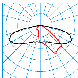
LIQ 50N-AB2L-SLR1/2200-730 2G1 ET (CLO initial value) TX277705 DIN 5040: A30 UTE: 1,00 G CEN Flux Code: 34 71 96 100 100 0 0 0 0 ■ C0 - C180 ■ C90 - C270
